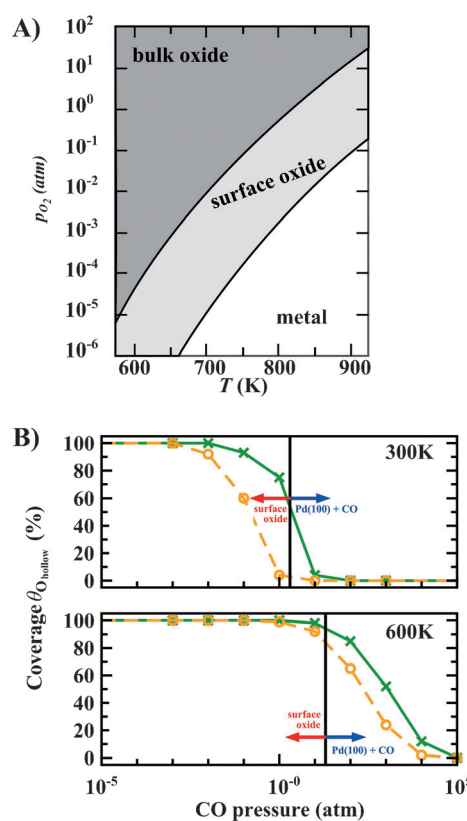
Figure 22. A) The calculated stability range of Pd bulk metal, surface oxides at Pd(100), and PdO bulk oxide at various T and p (Refs. [167,168]). B) Average occupation of hollow sites by oxygen versus CO pressure for T=300 K and T=600 K (from Ref. [169]). The vertical black line marks the boundary between the surface oxide and a CO-covered Pd(100) surface as determined within the constrained thermodynamics approach. The influence of the barrier on the O hollow + CO bridge → CO 2 reaction is illustrated by showing the kMC simulation results for two barrier values of 0.9 eV (green) and 0.8 eV (orange), see text.
