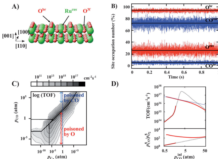
Figure 21. A) Surface structure of RuO_2(110) under UHV conditions as predicted by DFT calculations and observed experimentally. If we ignore relaxations, this is essentially a truncated bulk geometry. The bridge sites (occupied by O^{br} ), the naked Ru^{cus} atoms (cus = coordinatively unsaturated site), and the second layer threefold (3f) coordinated O^{3f} atoms are labeled. B) Time evolution of the occupation of the two prominent adsorption sites, bridge and cus, by O atoms and CO molecules. The assumed temperature and pressure conditions ( T = 600 K, p_{CO} = 7 atm, p_{O_2} = 1 atm) correspond to the optimum catalytic performance. Under these conditions a kinetic steady-state surface population is built up in which O and CO compete for both types of sites at the surface. The fluctuations in the site occupations within the (20 \times 20) simulation cell are significant. Note the time range for the “induction period” until the steady-state populations are reached when starting from a fully oxygen-covered surface. C) Map of calculated TOFs at T = 600 K. The plot is based on 400 kMC simulations for different ( p_{CO}, p_{O_2} ) conditions. D) Comparison of intrinsic TOFs (blue dotted line, see text) with observable TOFs (red solid line) for the CO oxidation at RuO_2(110) in a stagnation flow reactor. At the high TOFs reached at the nominal inlet temperature of 600 K, the observable TOF is for most pressures very close to the upper limit set by mass transfer through the boundary layer of products above the surface (blue line). This limit is a reactor property, independent of the employed catalyst. (From Ref. [25].)
